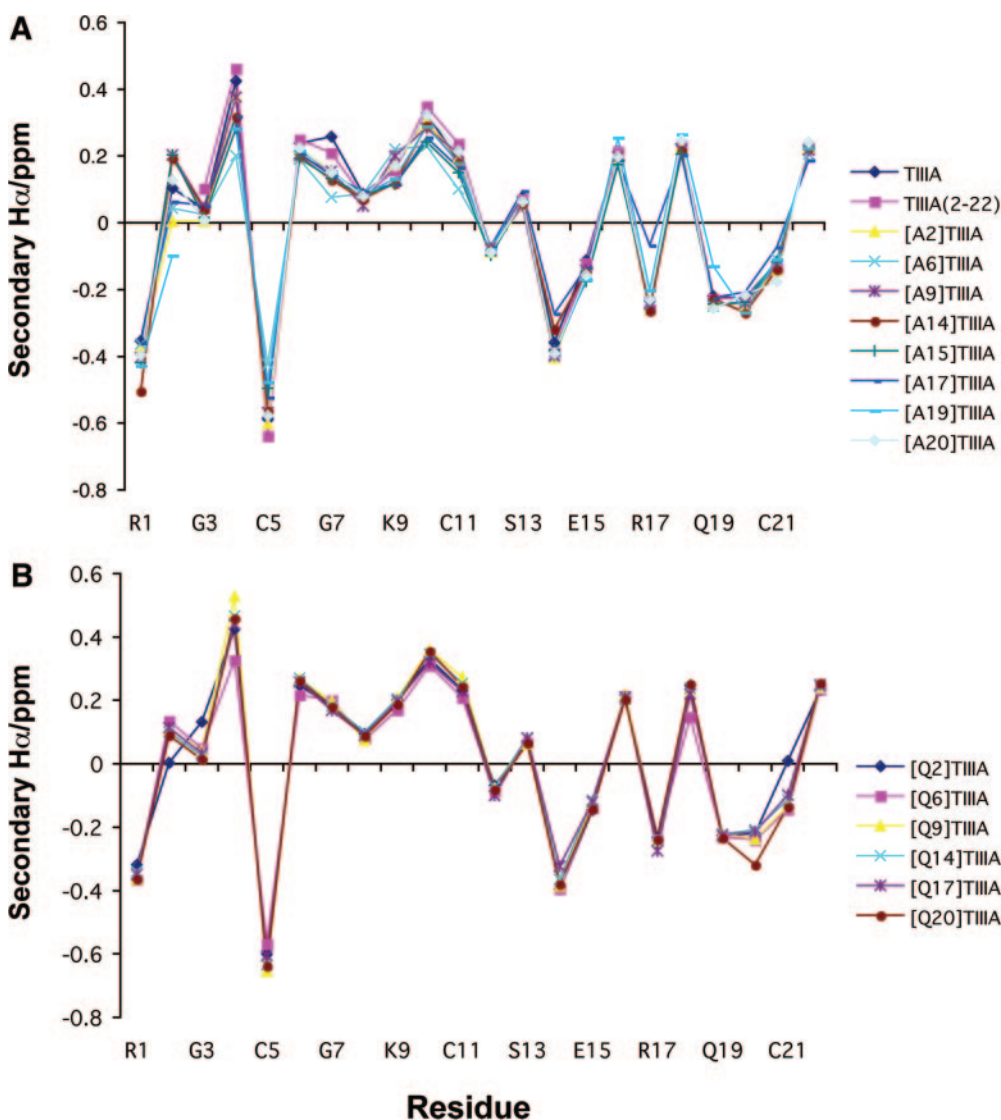
Fig. 4. Secondary H \alpha shifts of TIIIA and analogs. A, TIIIA compared with TIIIA(2–22) and Ala-substituted analogs. B, comparison of TIIIA and Gln-substituted analogs.
