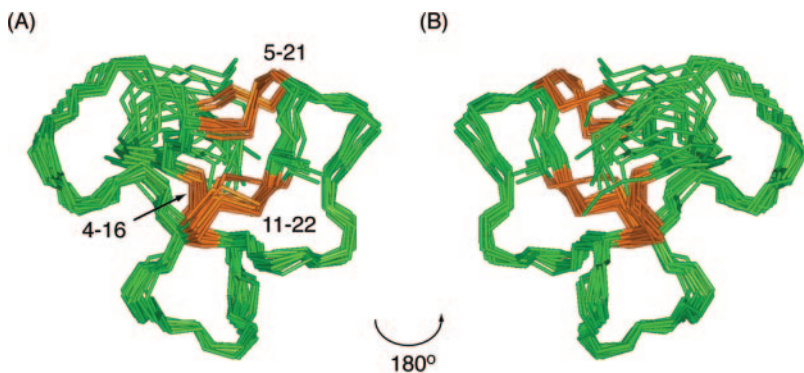
Fig. 7. Structure of TIIIA. A, backbone superimposition over the region 3 to 22 for the 20 lowest energy structures. B, 180° rotation of the structures shown in A, with the disulfide bridges indicated in orange.
