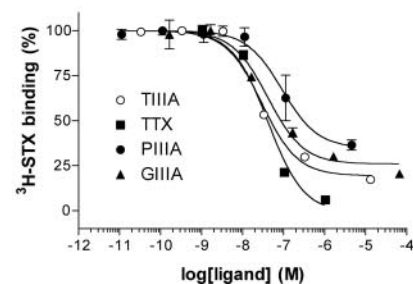
Fig. 1. Displacement of site 1 toxins from VGSCs. A, saturation binding curve for ^{125}\text{I} -TIIIA on rat brain VGSCs. Displacement of ^{125}\text{I} -TIIIA from rat brain (B) and rat skeletal muscle VGSCs (C). Displacement of [ ^3\text{H} ]STX from rat brain (D) and rat skeletal muscle VGSC (E).
